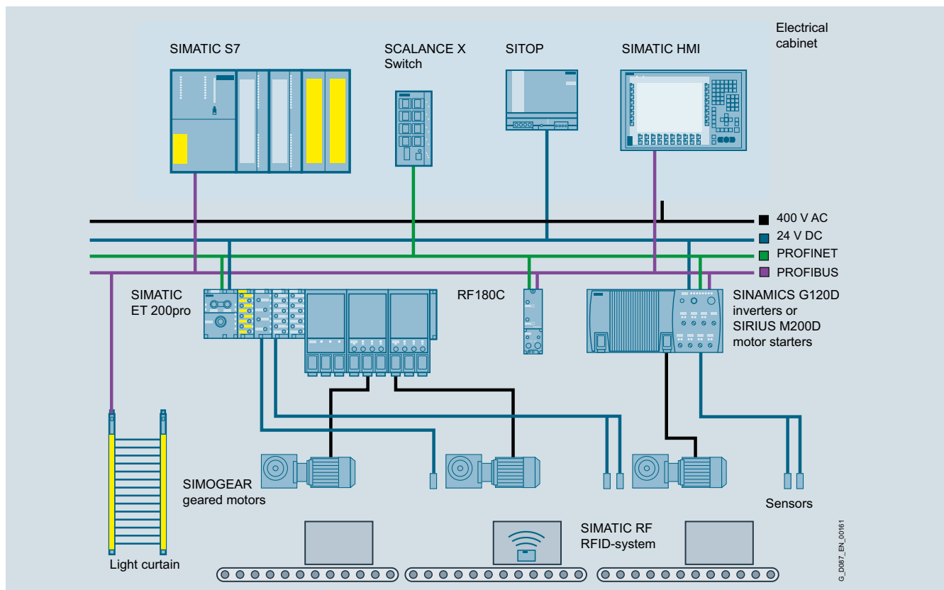
Fig. 1/8 Example of the Siemens Integrated Drive System (IDS) for sophisticated conveyor applications
