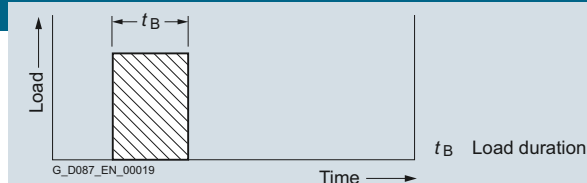
Fig. 2/6 Duty type S2
