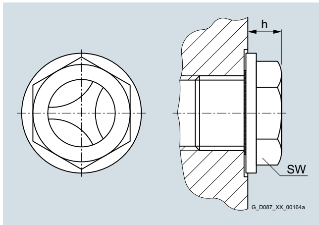
Fig. 10/19 Oil sight glass
