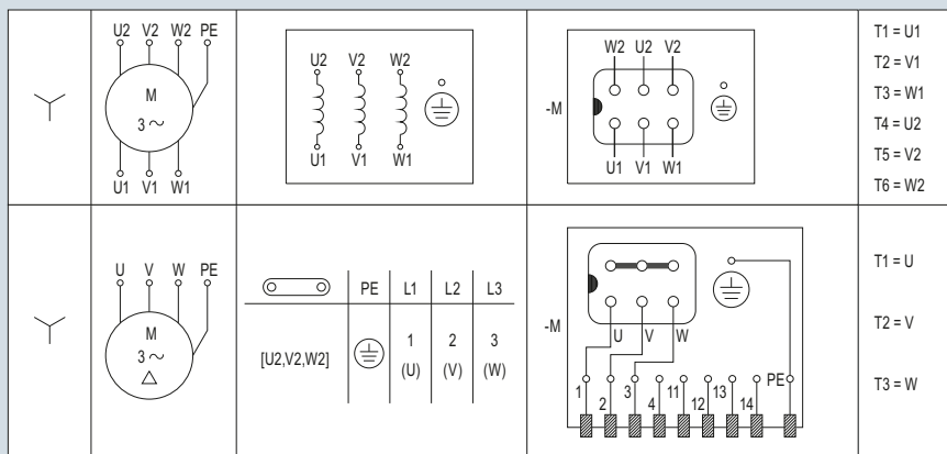
Fig. 11/19 Connection circuit diagram for motor winding Y connection
