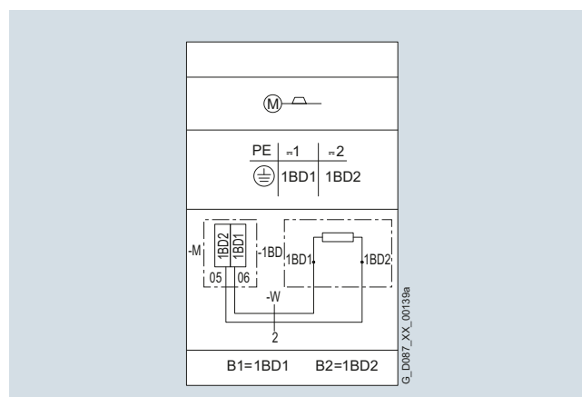
Fig. 11/35 Connection circuit diagram with DC control voltage
