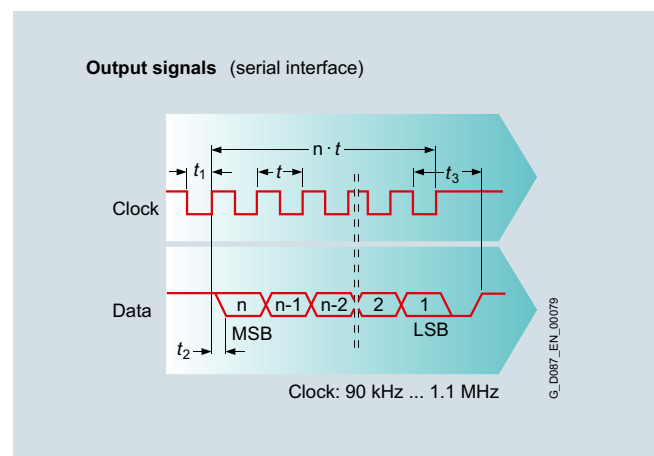
Fig. 2/26 Output signals
