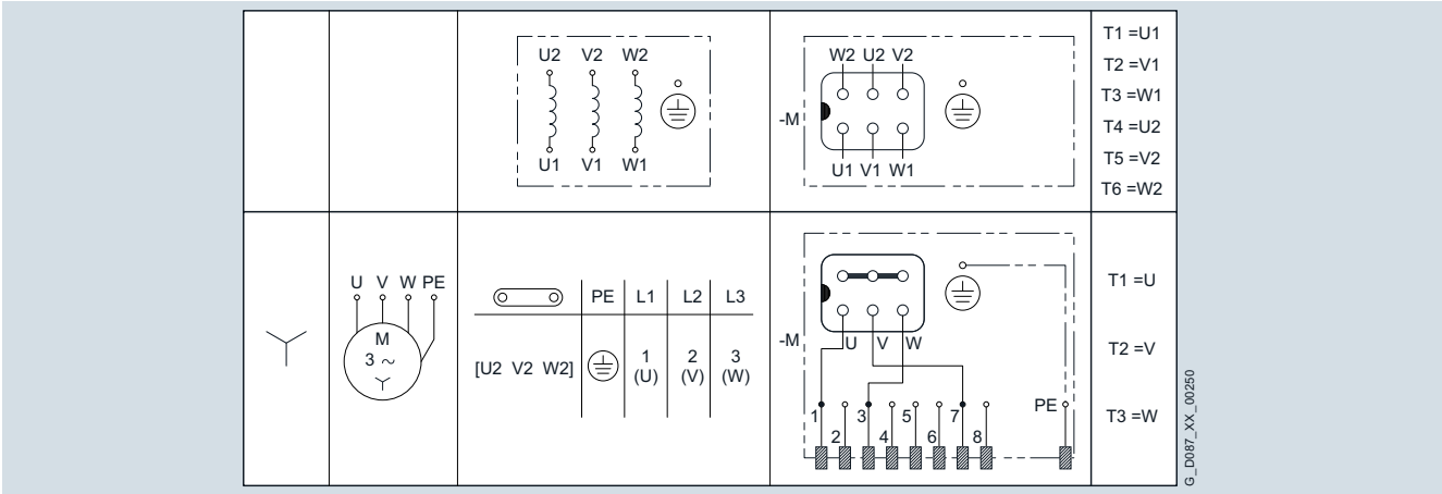
Fig. 11/23 Connection circuit diagram for motor winding Y connection
