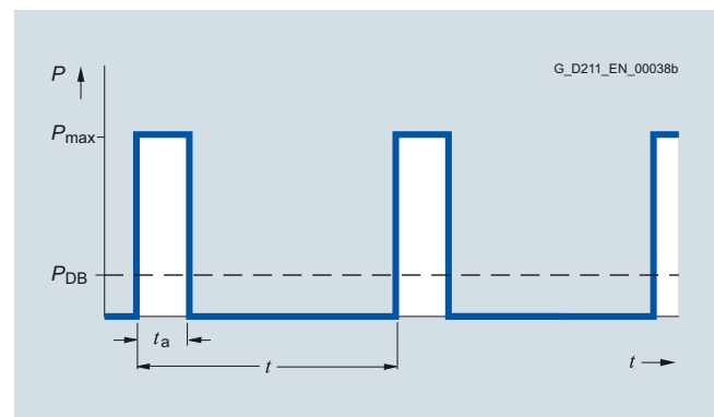
Fig. 9/23 Load diagram for the braking resistors t_a = 12 s t = 120 s
