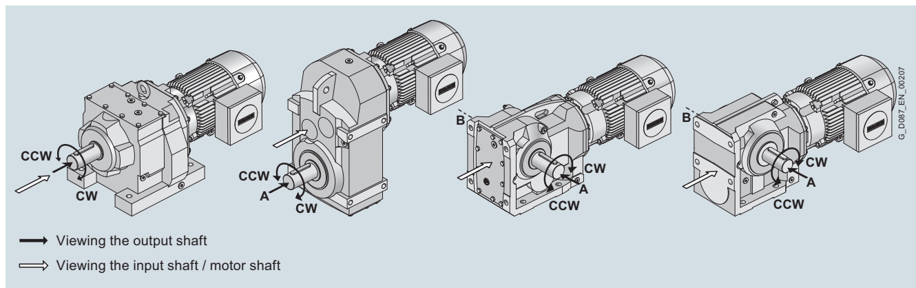
Fig. 1/18 Definition of the direction of rotation
