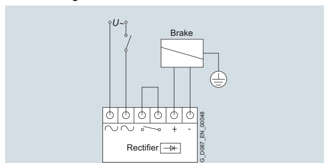
Fig. 11/36 Function diagram of a brake switched on the AC side
