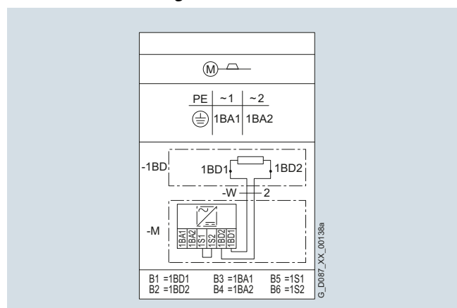
Fig. 11/34 Connection circuit diagram with AC control voltage
