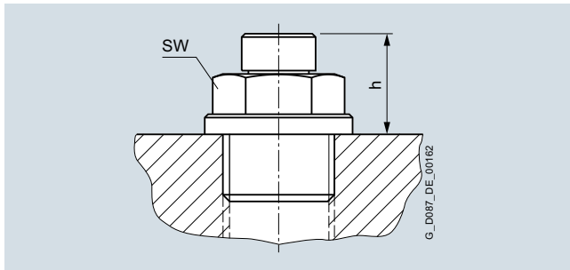
Fig. 10/15 Pressure breather valve
