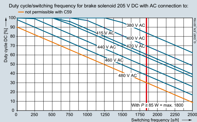
Fig. 11/39 Duty cycle/switching frequency for the 205 V DC brake solenoid
