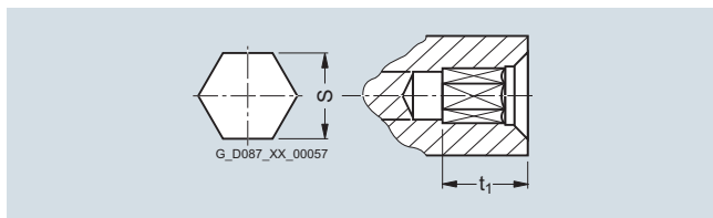
Fig. 11/61 Hexagonal recess
