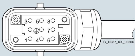
Fig. 11/26 Pin assignments for motor plug with 0.5 m cable, plug insert rotated by 180°
