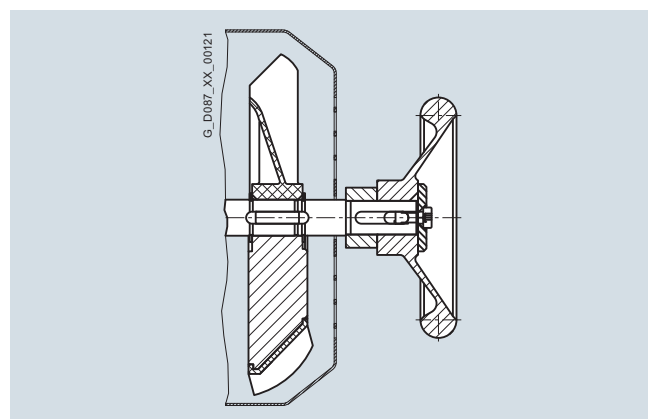
Fig. 11/60 Handwheel
