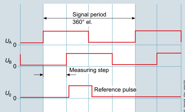
Fig. 2/21 Output signals
