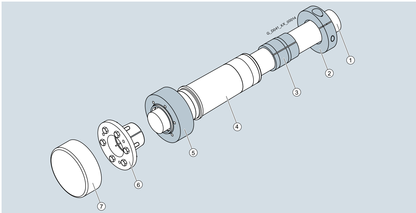
Fig. 10/14 SIMOLOC assembly system
