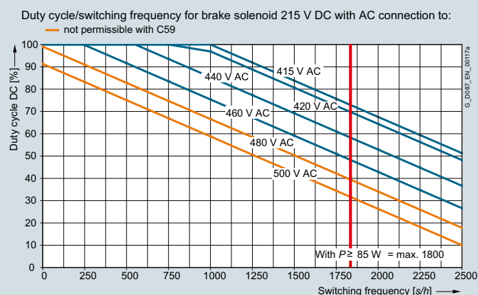
Fig. 11/40 Duty cycle/switching frequency for the 215 V DC brake solenoid
