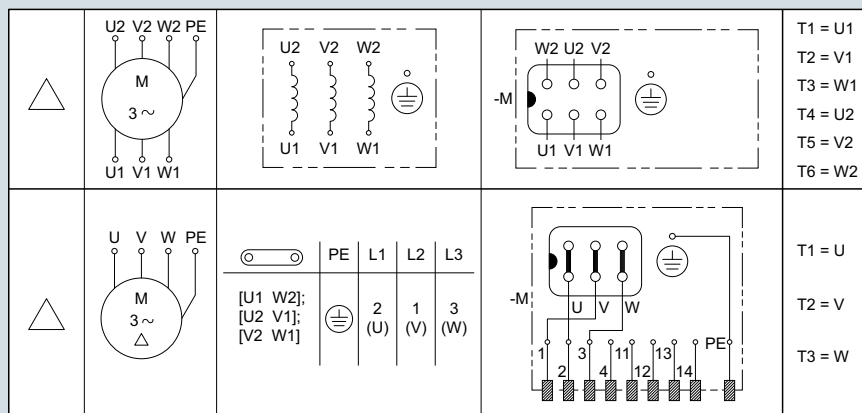
Fig. 11/20 Connection circuit diagram for motor winding Δ connection
