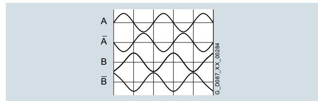
Fig. 11/53 Chart pattern with shaft rotating in clockwise direction (looking in direction of clamping ring)
