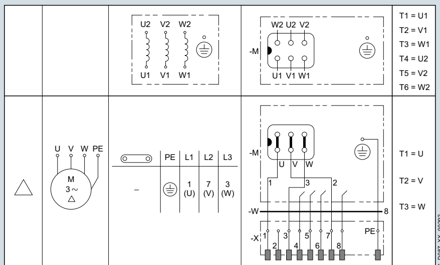
Fig. 11/29 Connection circuit diagram for motor winding Δ connection
