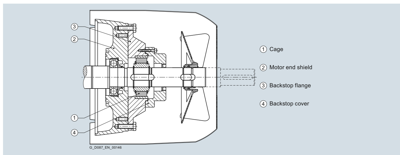
Fig. 11/58 Backstop
