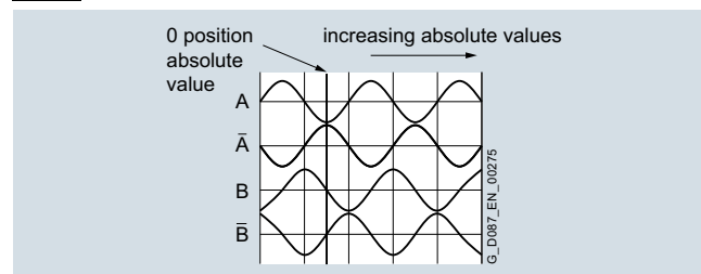
Fig. 11/55 Chart pattern with shaft rotating in clockwise direction (looking in direction of clamping ring)
