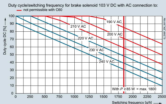
Fig. 11/38 Duty cycle/switching frequency for the 103 V DC brake solenoid
