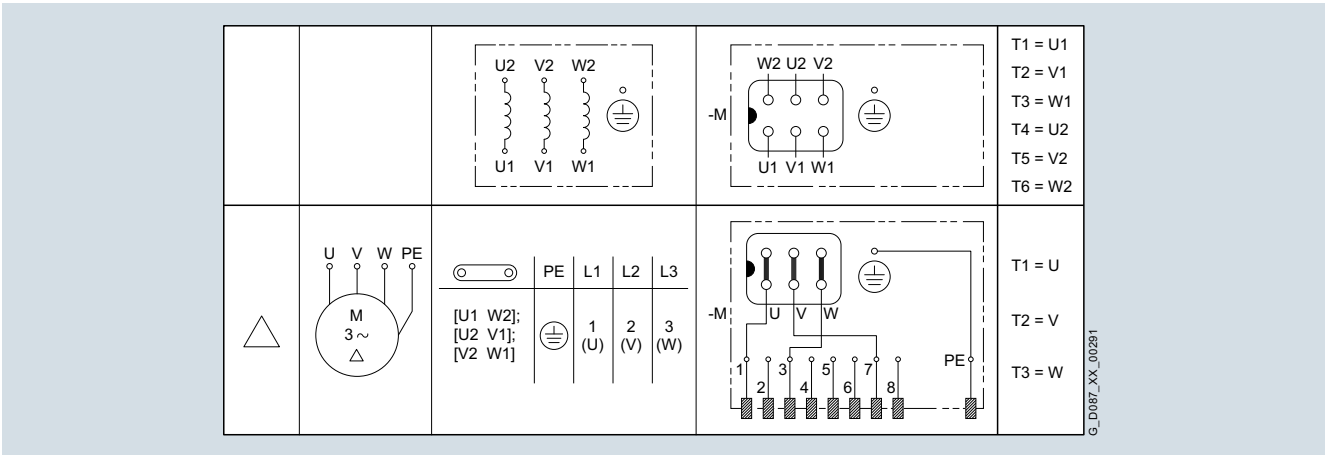
Fig. 11/24 Connection circuit diagram for motor winding Δ connection
