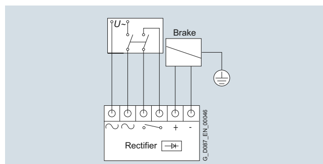
Fig. 11/37 Function diagram of a brake switched on the DC and AC sides
