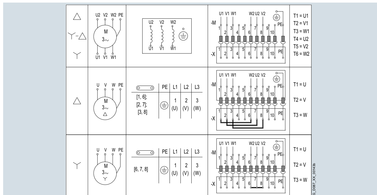
Fig. 11/17 Connection circuit diagram for motor winding
