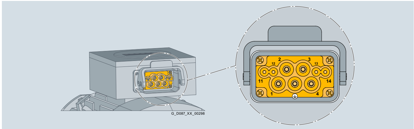
Fig. 11/18 HAN K4/4 motor plug with pin assignments
