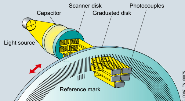
Fig. 2/20 Principle of operation, photoelectric scanning
