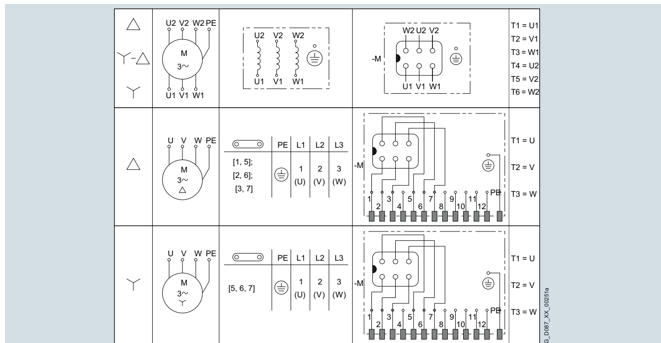
Fig. 11/31 Connection circuit diagram for motor winding
