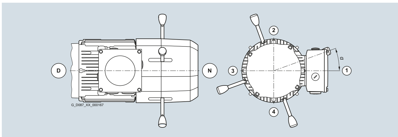
Fig. 11/43 Manual brake release lever position
