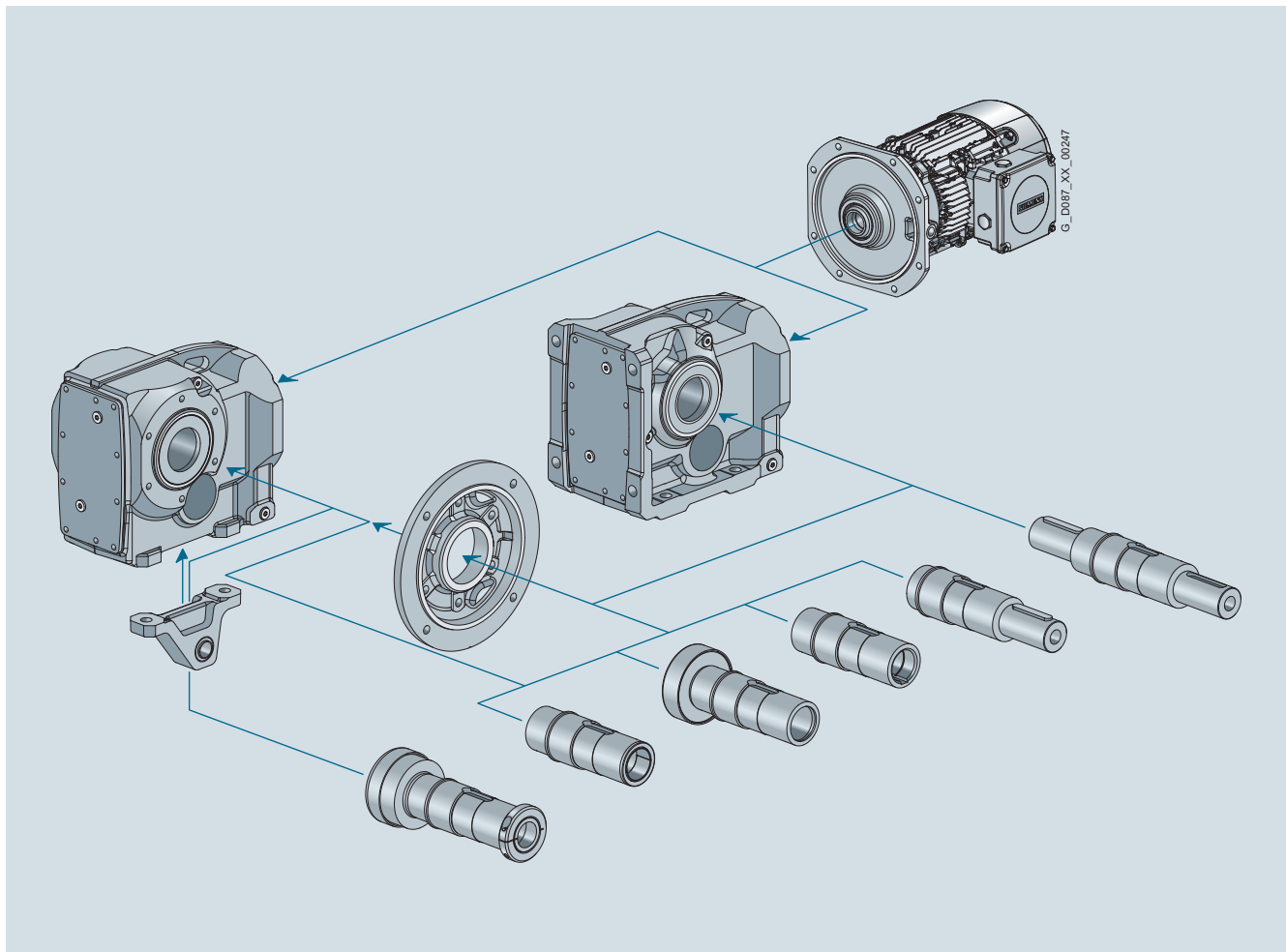
Fig. 1/13 Modular system, bevel geared motor K
