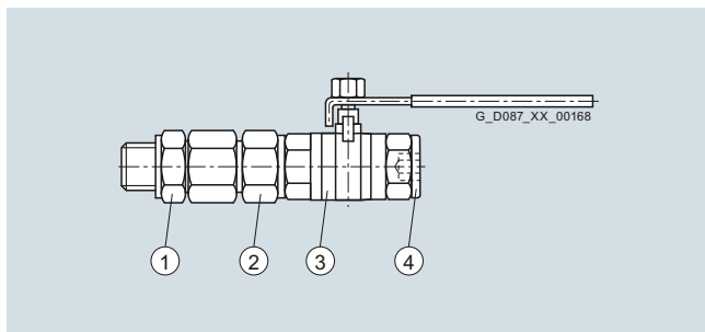
Fig. 10/20 Oil drain valve, straight
