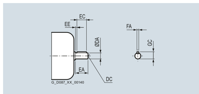
Fig. 11/59 Second motor shaft extension
