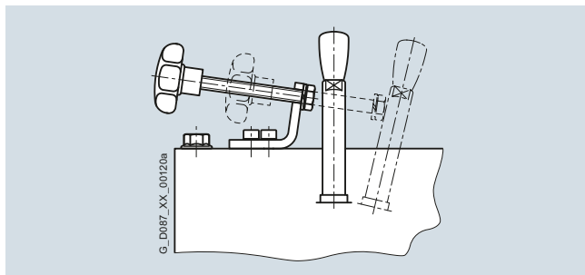
Fig. 11/41 Example of manual brake release lever with locking mechanism for brake L
