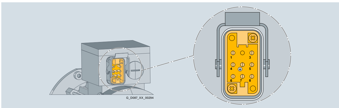
Fig. 11/21 HAN Q8 motor plug with pin assignments for motor frame sizes 63 and 71
