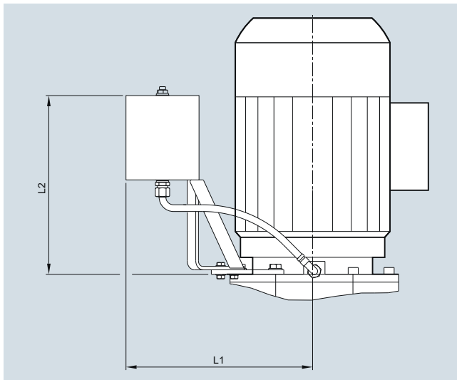
Fig. 10/17 Oil expansion unit type 2
