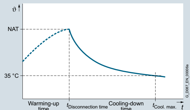
Fig. 11/4 Temperature switch characteristic
