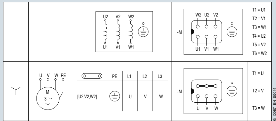
Fig. 11/12 Connection circuit diagram, motor connection Y
