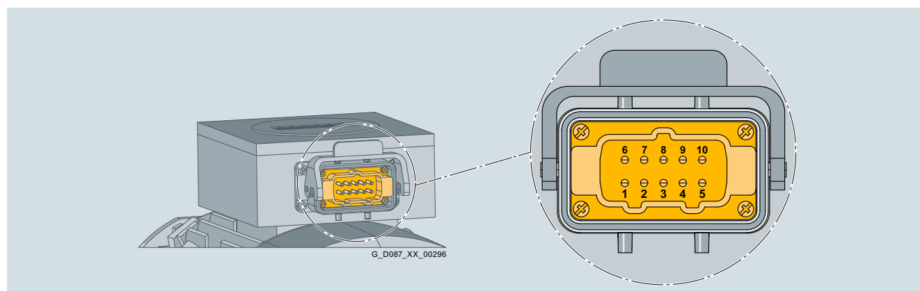
Fig. 11/16 HAN 10 E motor plug with pin assignments
