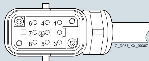
Fig. 11/27 Pin assignments for motor plug with 1 m to 5 m cable, plug insert rotated by 0°
