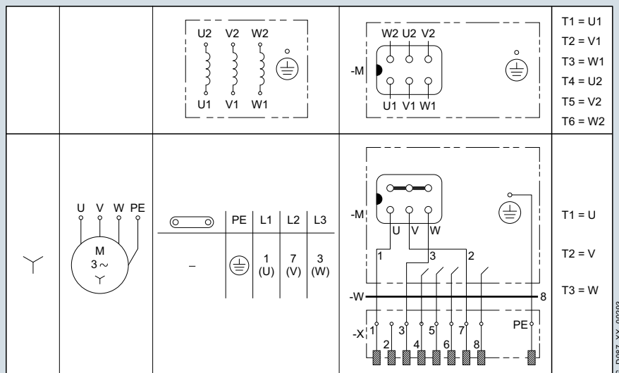
Fig. 11/28 Connection circuit diagram for motor winding Y connection
