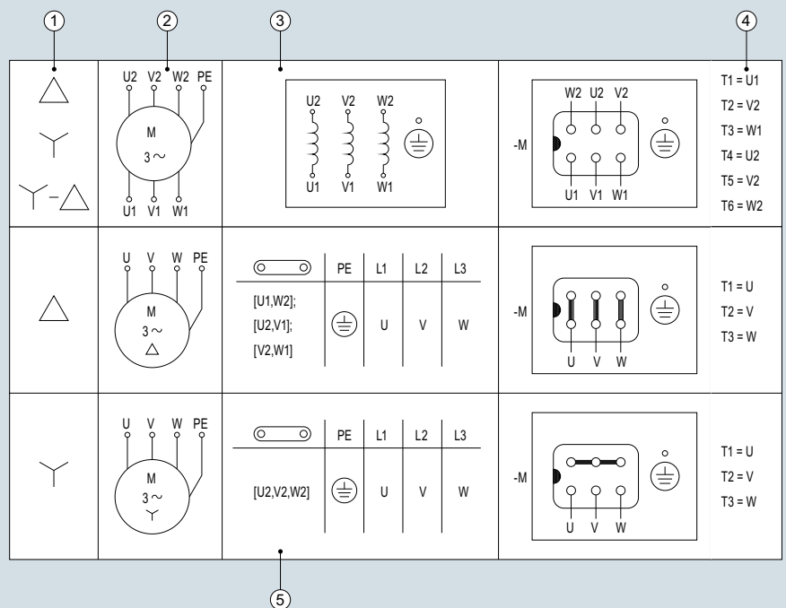
Fig. 11/11 Connection circuit diagram, motor connection Δ/Y
