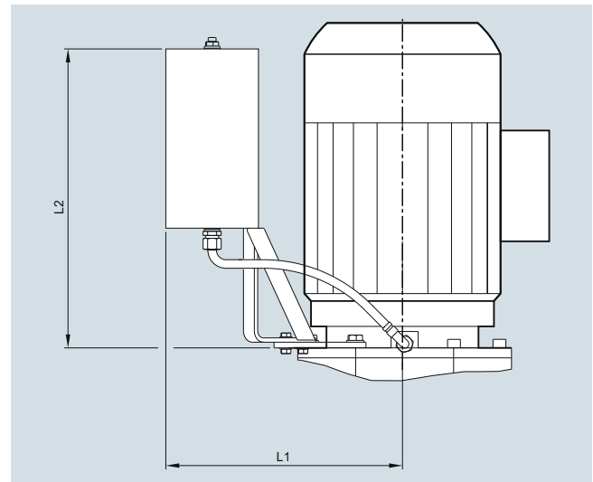
Fig. 10/18 Oil expansion unit type 3
