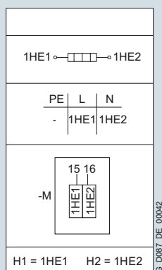
Fig. 11/9 Connection circuit diagram for the anti-condensation heating
