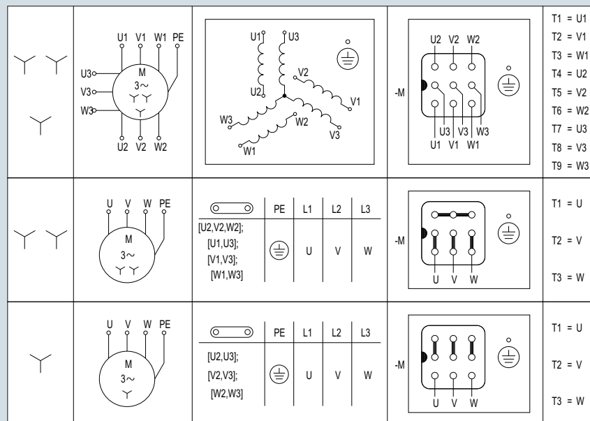
Fig. 11/13 Connection circuit diagram, motor connection YY/Y
