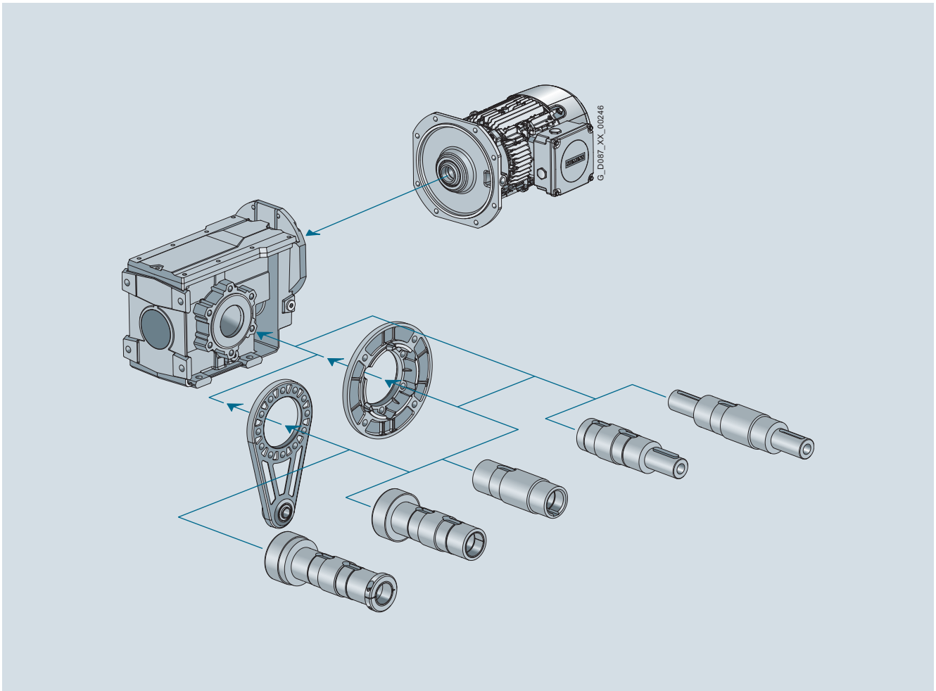
Fig. 1/12 Modular system, bevel geared motor B
