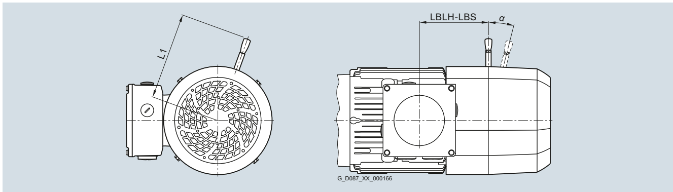
Fig. 11/44 Dimensions, manual brake release lever
