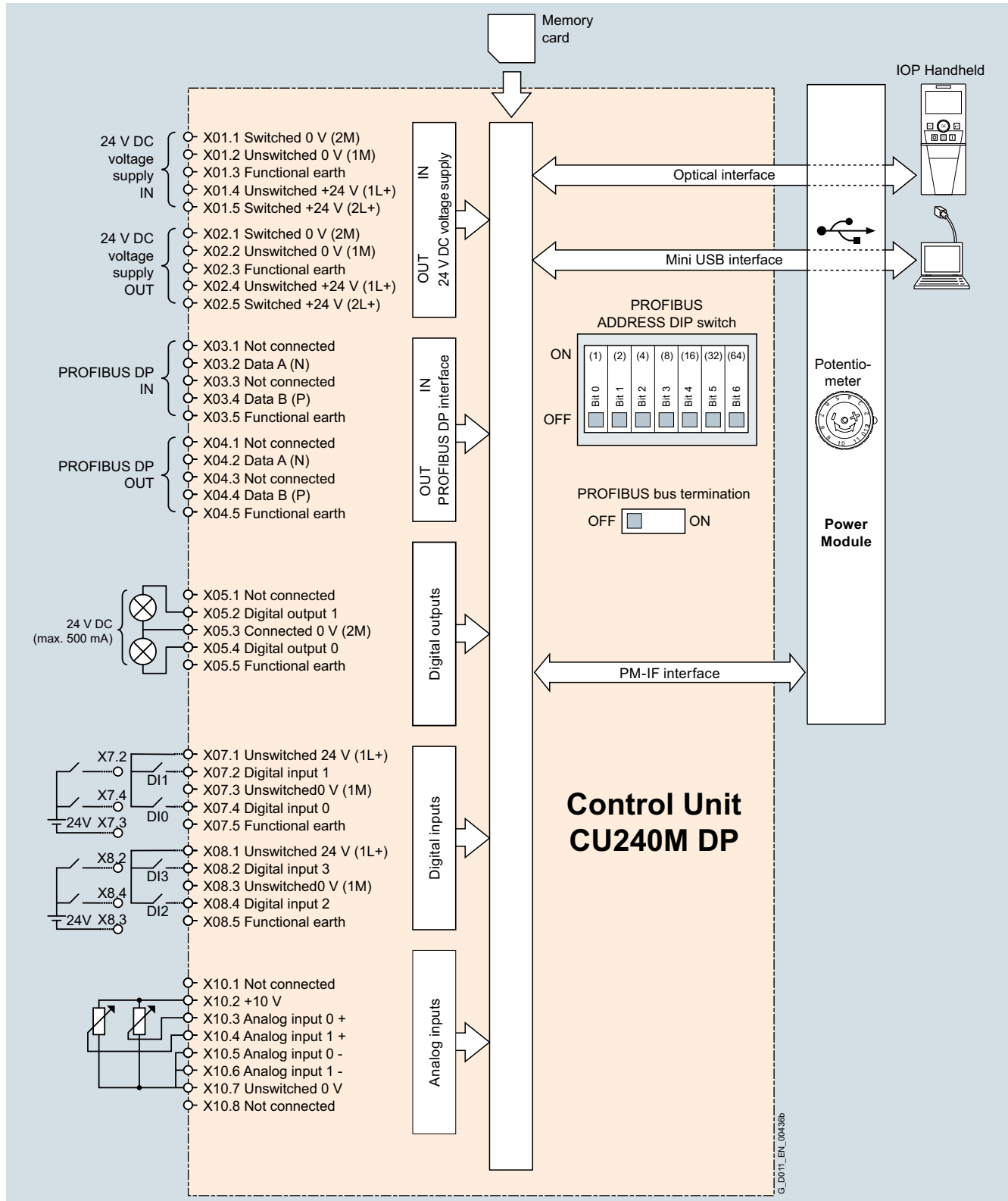
Fig. 9/11 Connection diagram for CU240M DP Control Units
