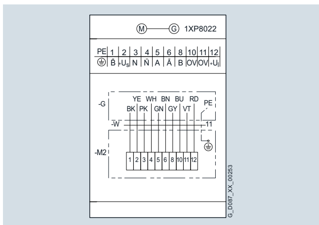
Fig. 11/57 Connection circuit diagram
