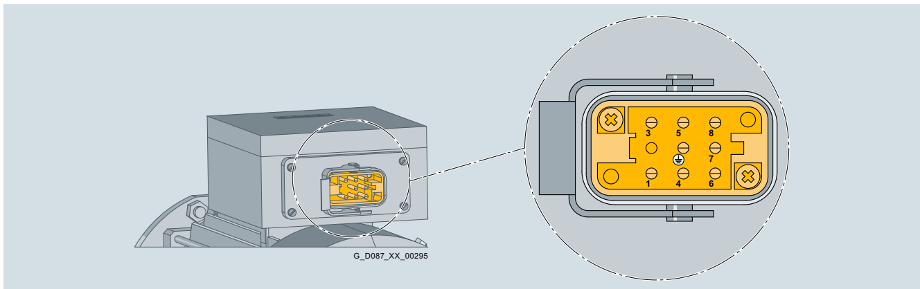
Fig. 11/22 HAN Q8 motor plug with pin assignments for motor frame sizes 80 to 132
