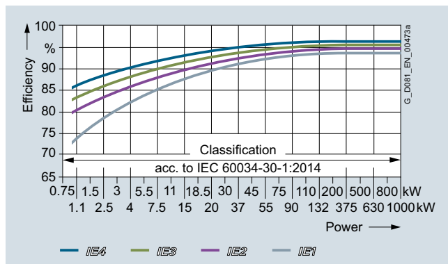
Fig. 1/17 IE1-IE3 efficiencies 4-pole at 50 Hz
