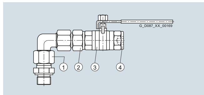
Fig. 10/21 Oil drain valve, angled
