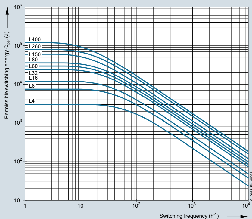
Fig. 11/46 Permissible operating energy
