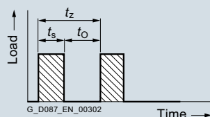
Fig. 2/19 Cyclic duration factor
